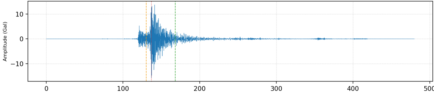
2. Filtered Ground Acceleration
